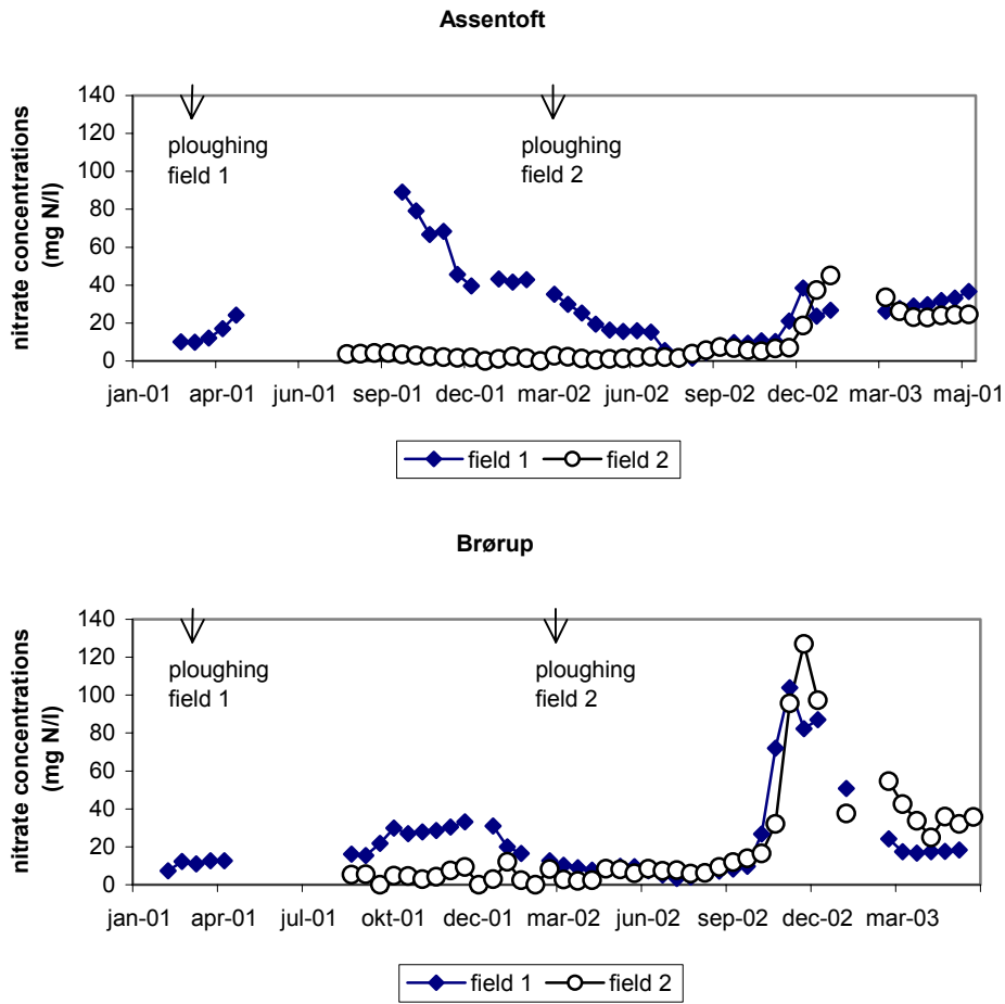
Figure 1. Concentrations of nitrate-N in soil water at a depth of 100 cm at a loamy sandy soil with moderate rainfall (Assentoft) and a sandy soil with high rainfall (Brørup).
